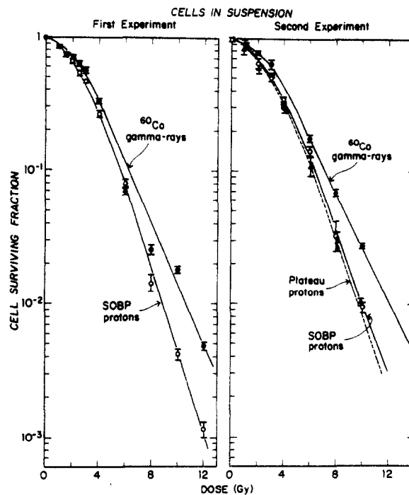
Fig. 5. Survival data for V79 Chinese hamster cells irradiated in suspension with ^{60}\text{Co} \gamma -rays or with protons in the spread-out Bragg peak (SOBP) or plateau positions of the depth dose profile (positions A or B respectively in Fig. 1). Two separate experiments were performed on different occasions. The curves were fitted to the data by a method described in the text.
